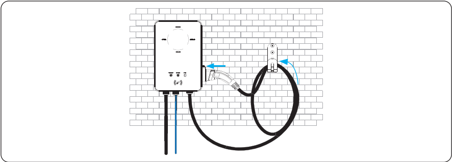
Figure 6-34 Connect the charging connector and hang the cable
