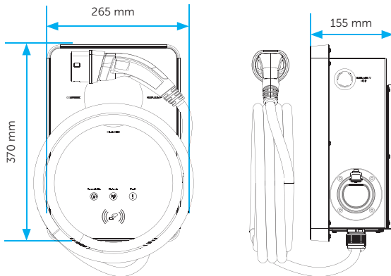
Figure 2-5 Dimensions of Plug Type
