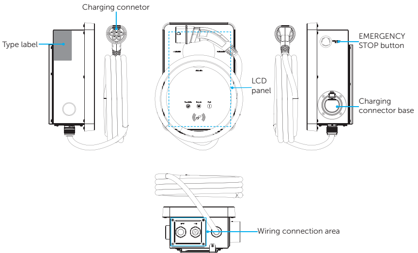
Figure 2-3 Appearance of Plug Type
