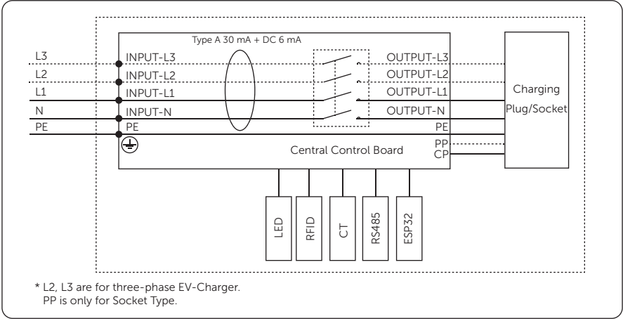
Figure 2-7 Principle Circuit Diagram
