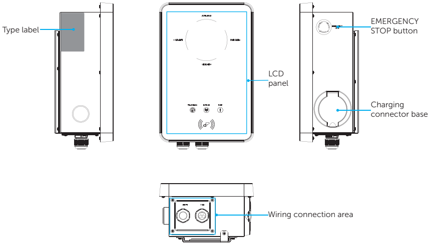
Figure 2-2 Appearance of Socket Type
