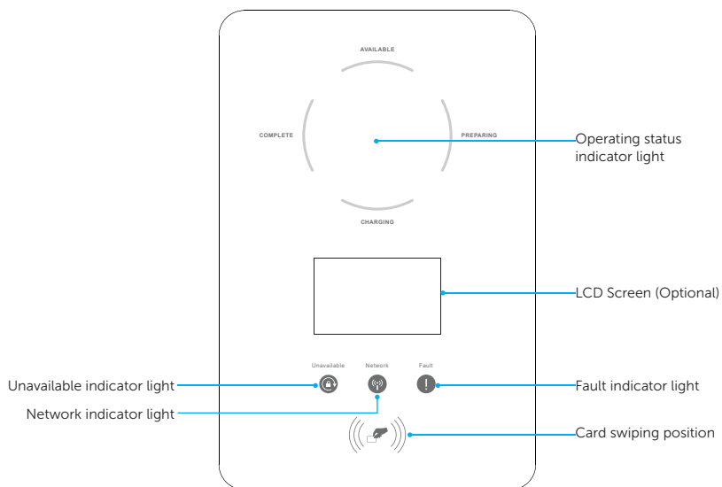
Figure 2-6 LCD Panel
