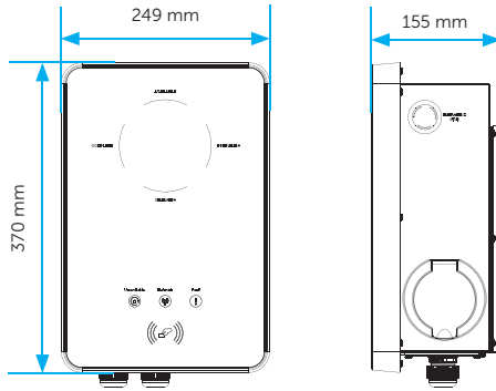
Figure 2-4 Dimensions of Socket Type
