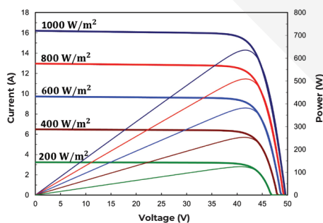
Current - Voltage & Power - Voltage Curve(PP640-132TNB12R)
