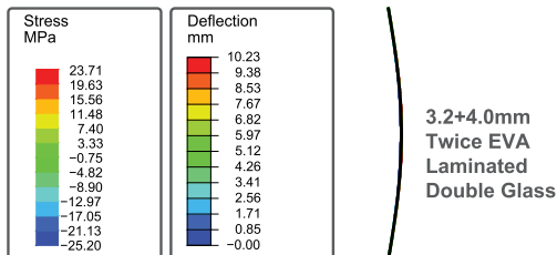
*Simulation Results Under 2400Pa Pressure
